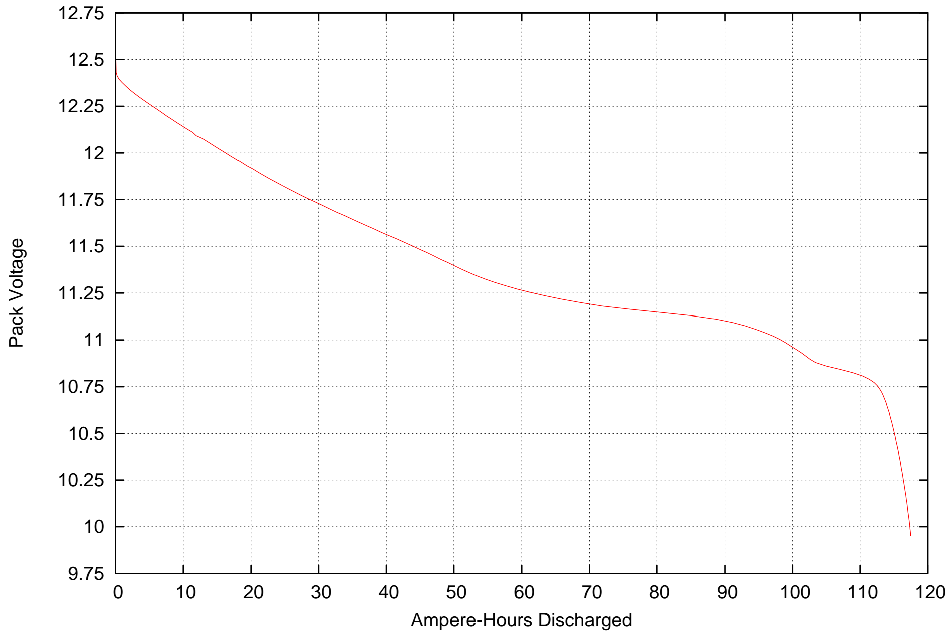
Genasun GL-105, Nominal C/20 Discharge (2 Ohm Load)
